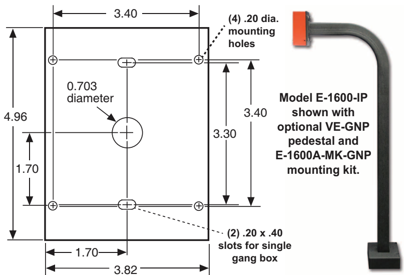
MOUNTING PLATE
